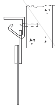
Some styles of fixing the hanging steel bar to the door frame
