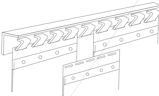
Some styles of fixing the hanging steel bar to the door frame
